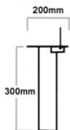
Ground socket for removable bollard
