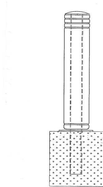
Resilient Bollard In Ground Fixed
